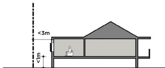
FFL above natural ground level >1m and distance to boundary is <3m Privacy screen required
