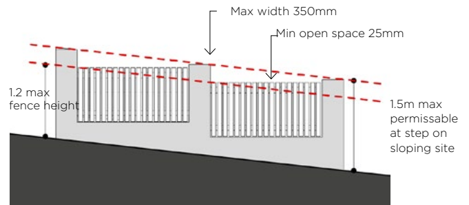
Figure 3-47 On sloping sites fences and walls should be stepped so that no part of the fence is higher than 1.5m above natural ground level
