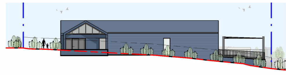
5 WESTERN ELEVATION 1 : 350
