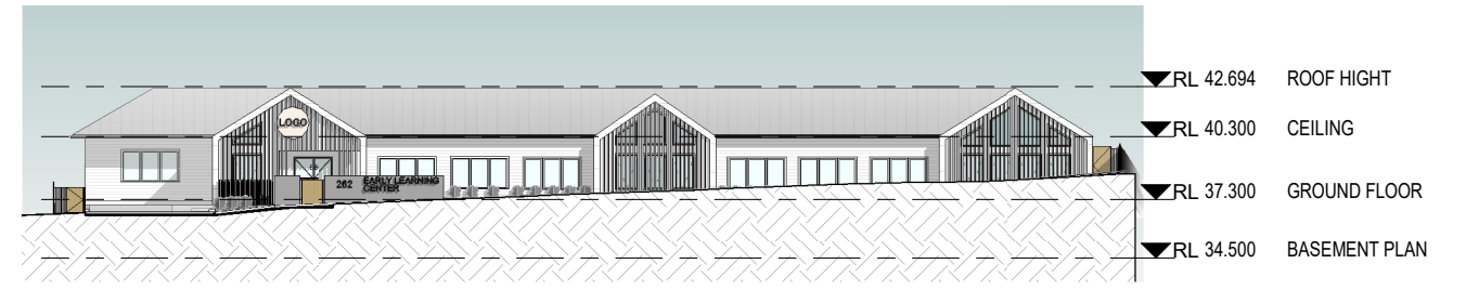
3 -WEST ELEVATION 1 : 350
