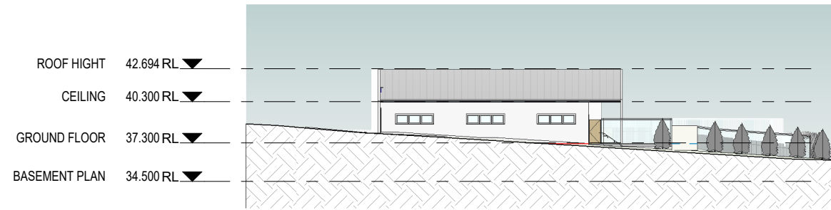
4 -SOUTH ELEVATION 1 : 350
