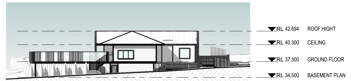
5 -NORTH ELEVATION 1 : 350
