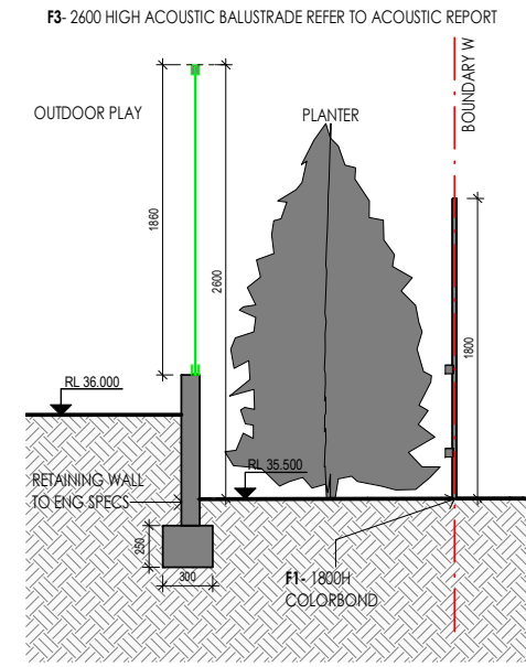
2 ACOUSTIC FENCE 1:25
